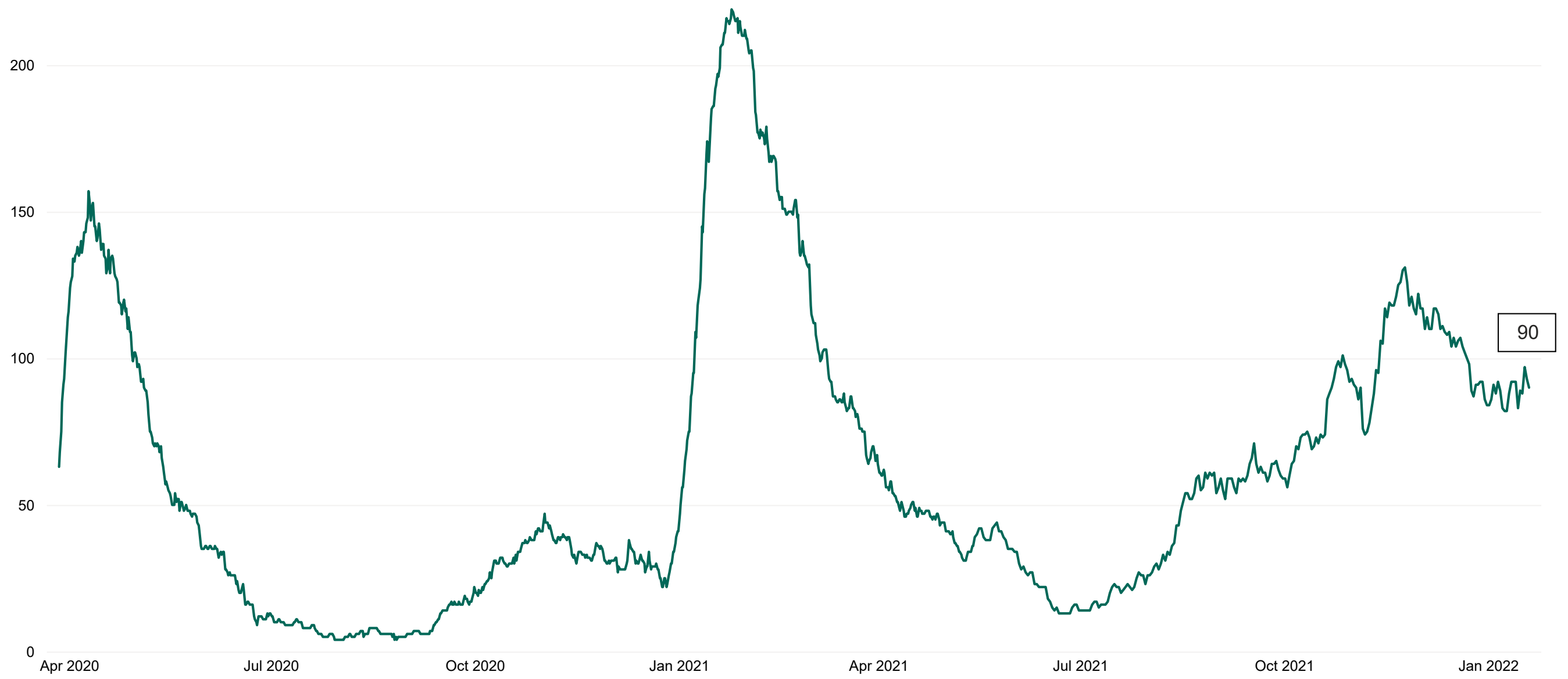
Confirmed COVID-19 Cases in ICU/HDU from 27/03/2020 to 19/01/2022
