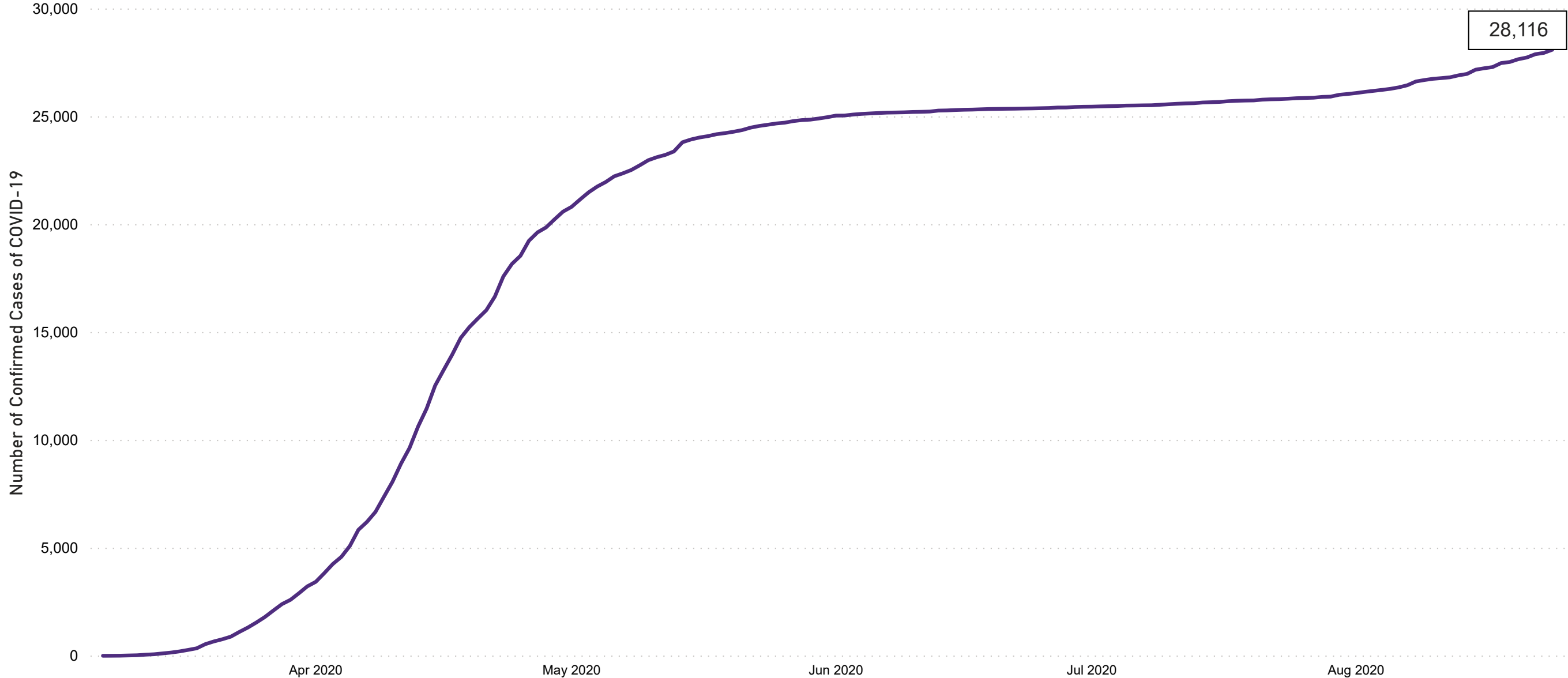
Confirmed Cases of COVID-19 in the Republic of Ireland as of 24/08/2020
