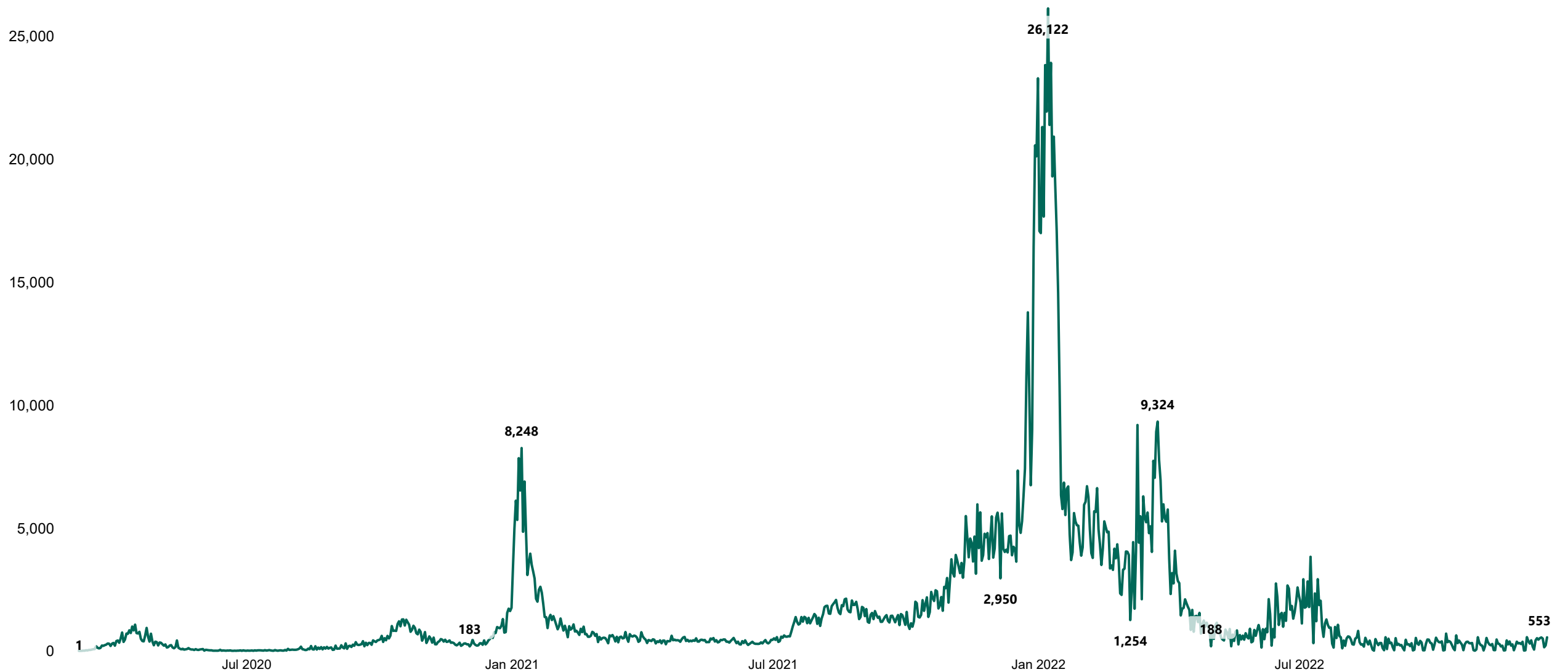
New Confirmed COVID-19 Cases in the Republic of Ireland as at 20/12/2022
