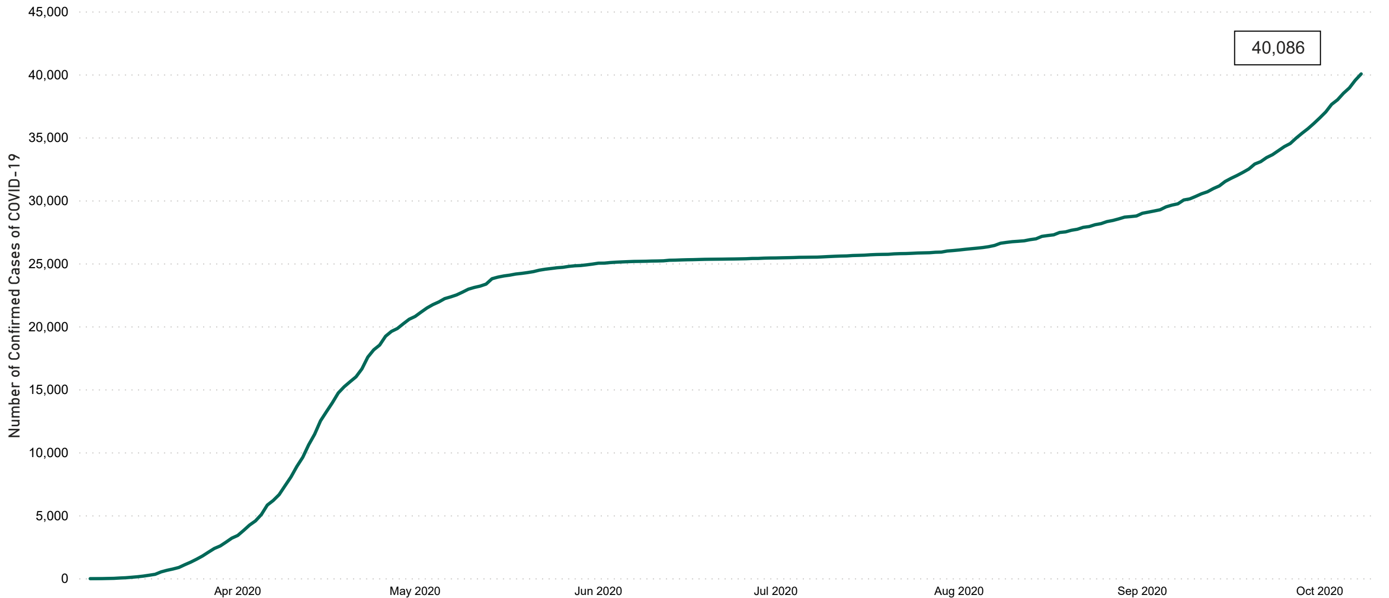
Confirmed Cases of COVID-19 in the Republic of Ireland as of 08/10/2020
