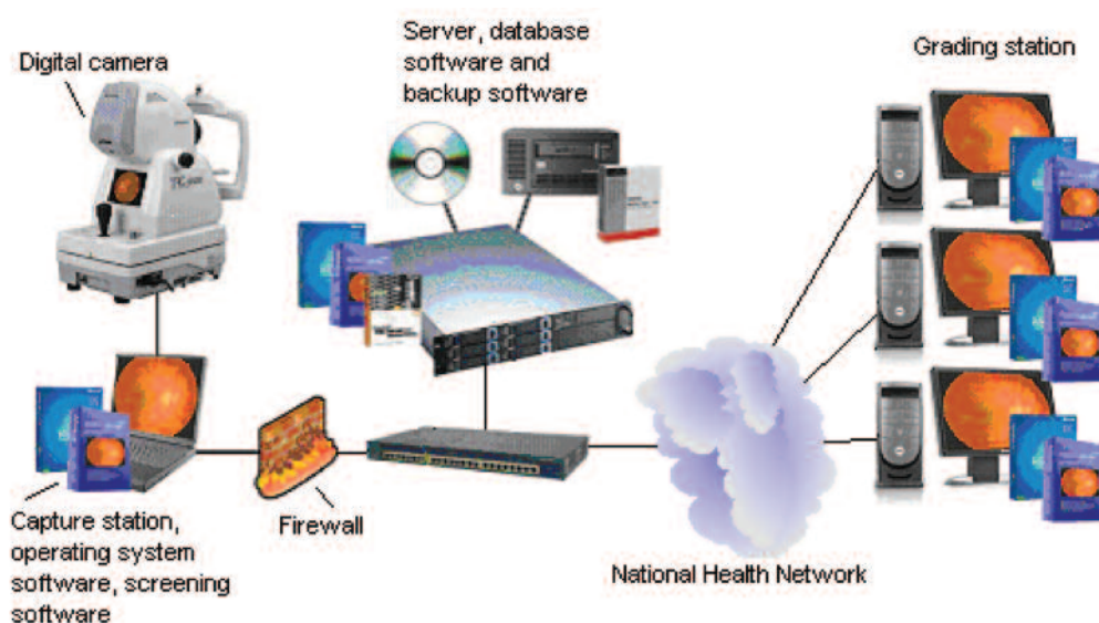
Figure 4: Hardware and software components of the proposed IT system
